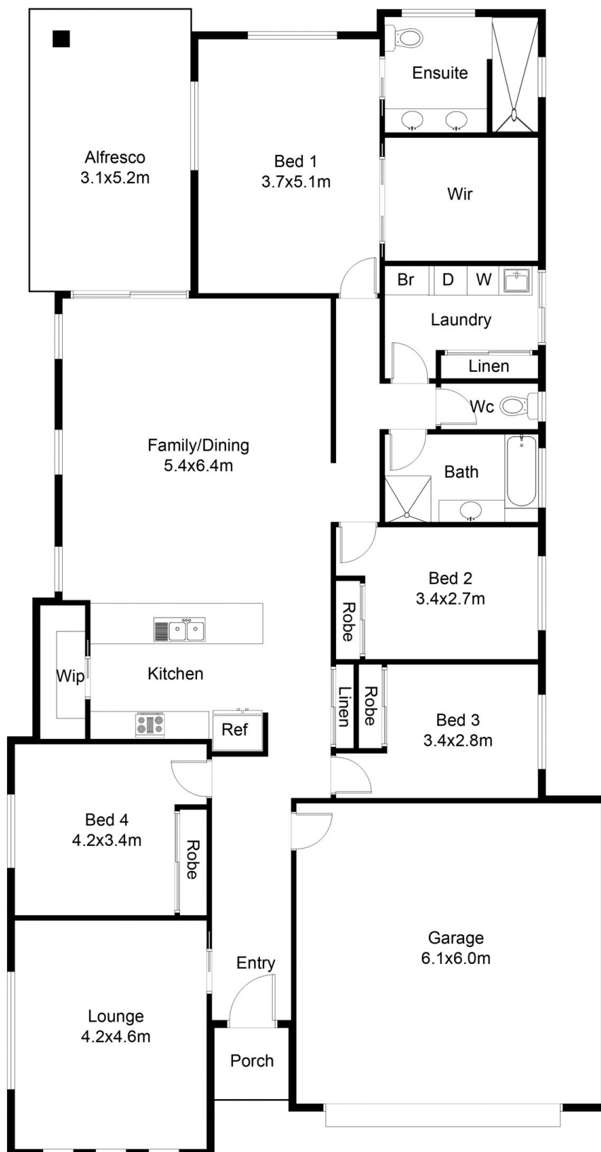
FLOOR PLAN
