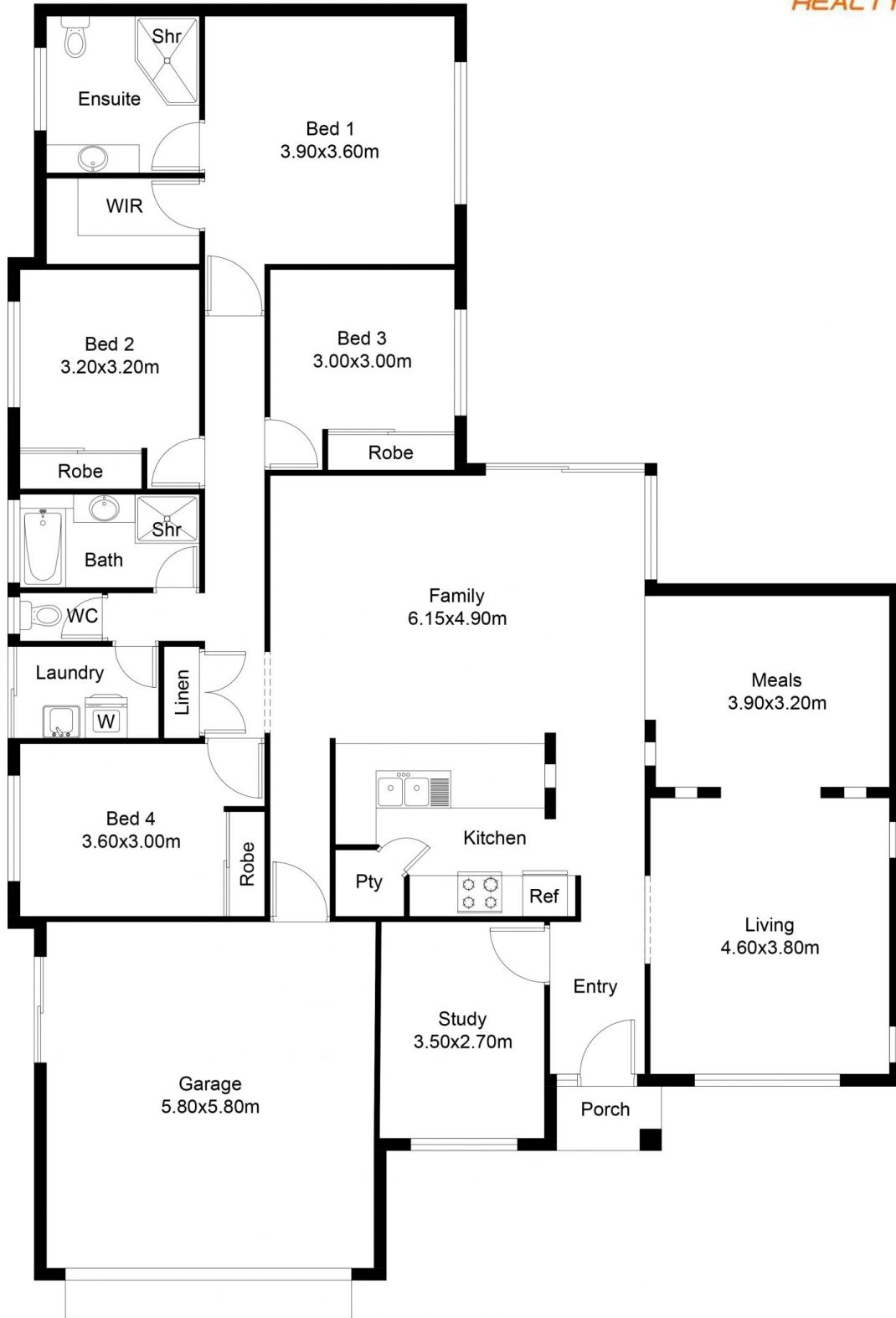
FLOOR PLAN
