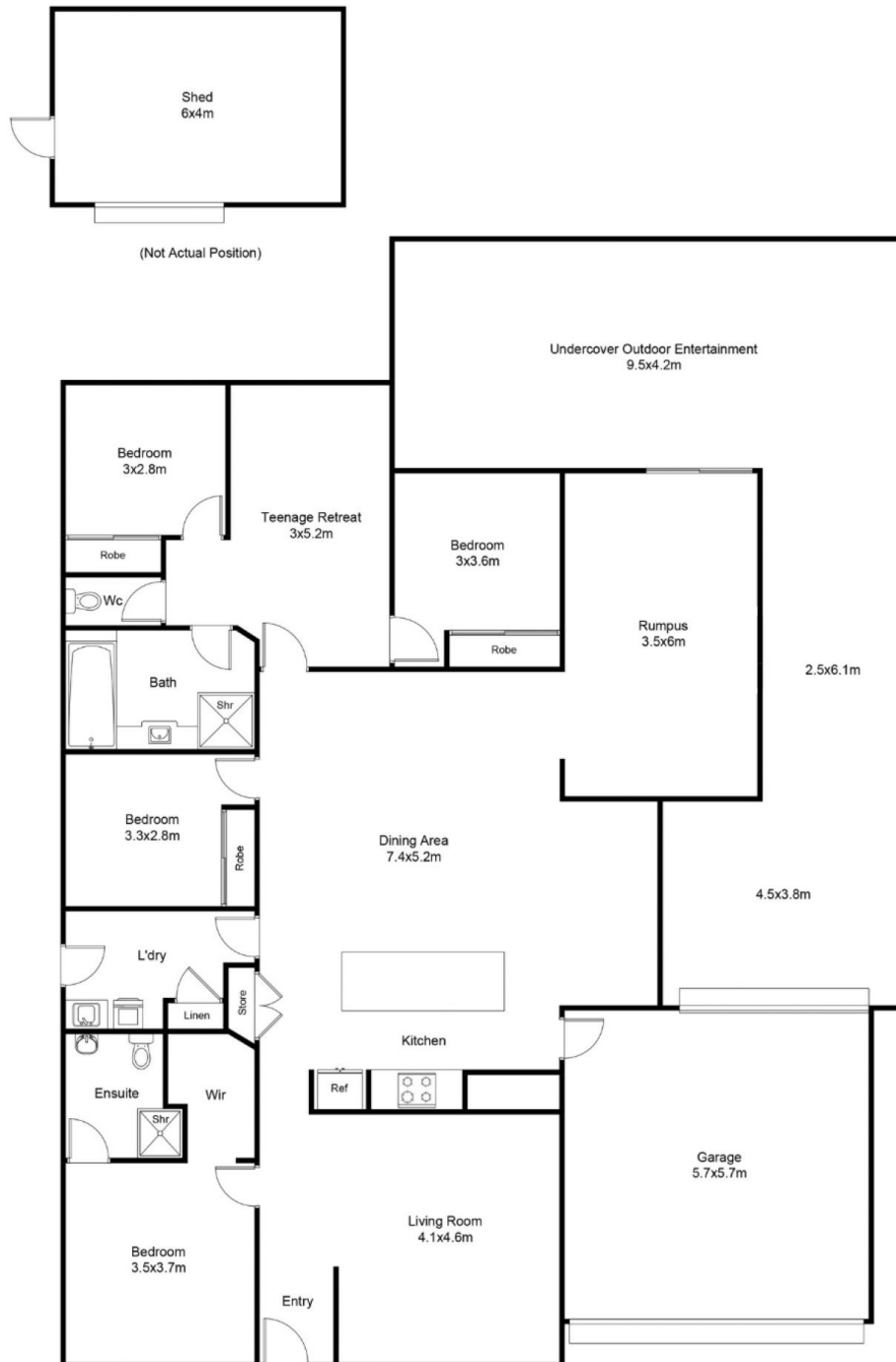
FLOOR PLAN
