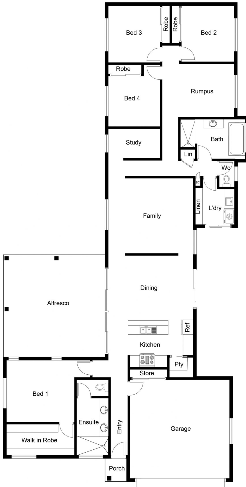
FLOOR PLAN
